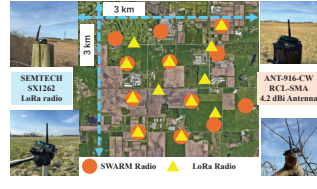
Figure 10: Outdoor deployment of flooding experiments and satellite radio locations.
